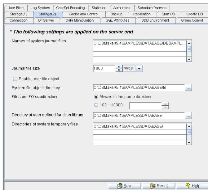
Figure 3-8 Storage (2) page
