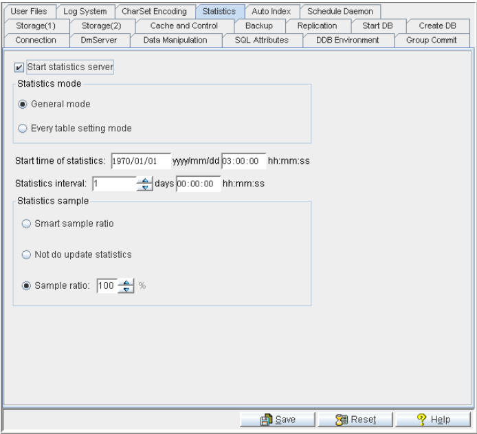
Figure 3-17 Statistics Page
