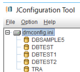
Figure 2-3 Tree Objects
