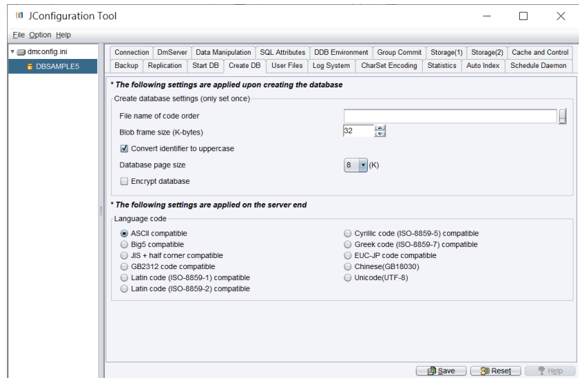
Figure 3-13 Create DB (database) Page
