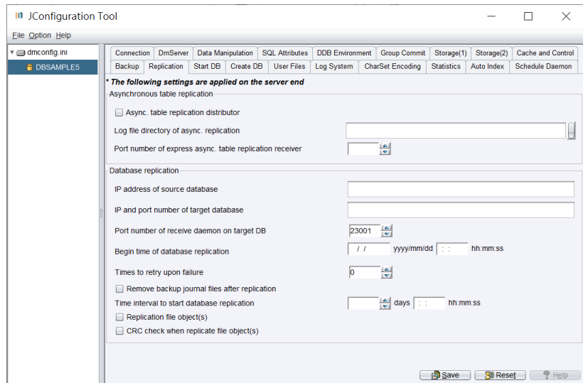
Figure 3-11 Replication Page
