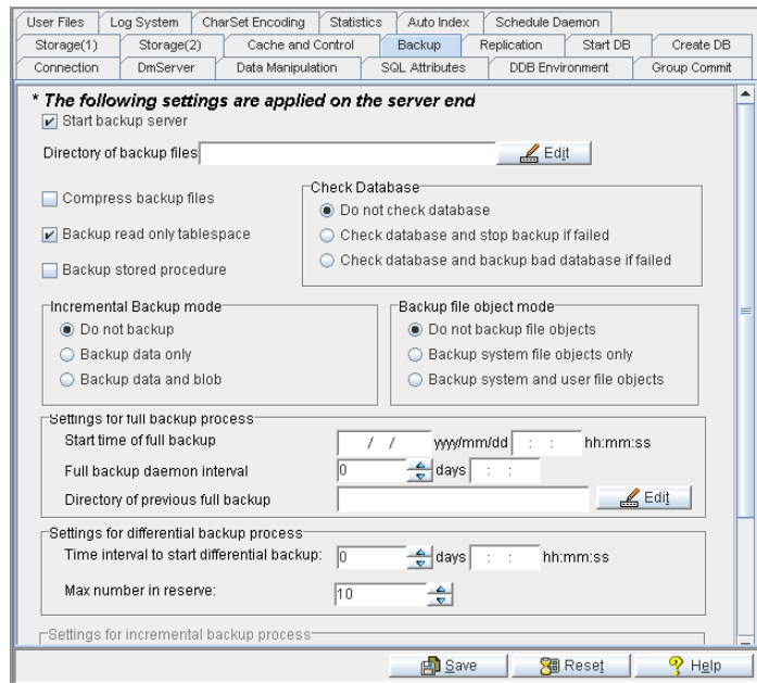
Figure 3-10 Backup Page
